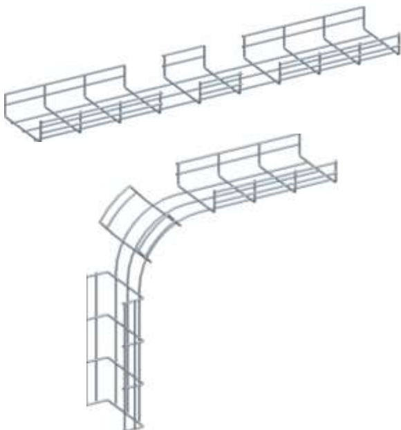
Vertical Bend Assembly Guide Vertical Inside and Outside Bends
