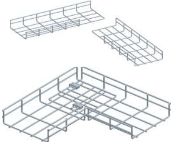
90° Bends Assembled From Two Straight Sections
